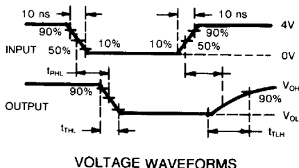
Figure 4 - Switching Times
