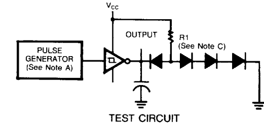
Figure 4 - Switching Times
