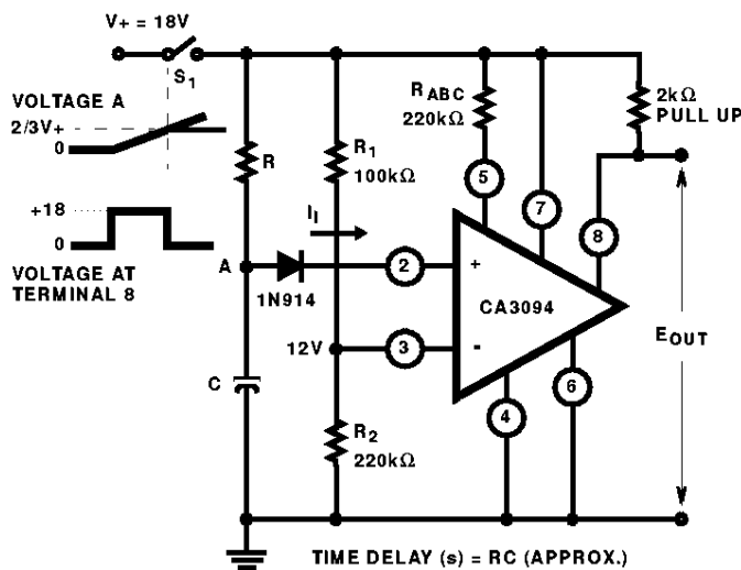
FIGURE 12. RC TIMER
