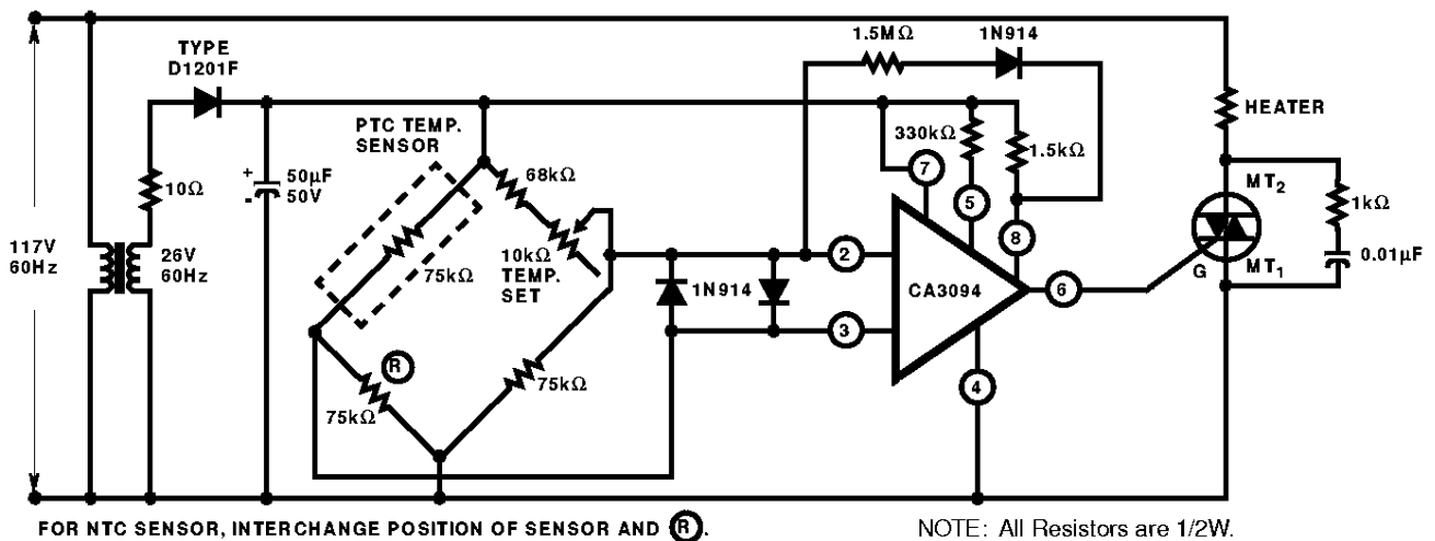
FIGURE 19. TEMPERATURE CONTROLLER
